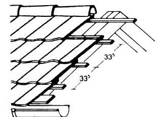
13 English slate roof with cement fibre boards, 0.45-0.55 kN/m 2
